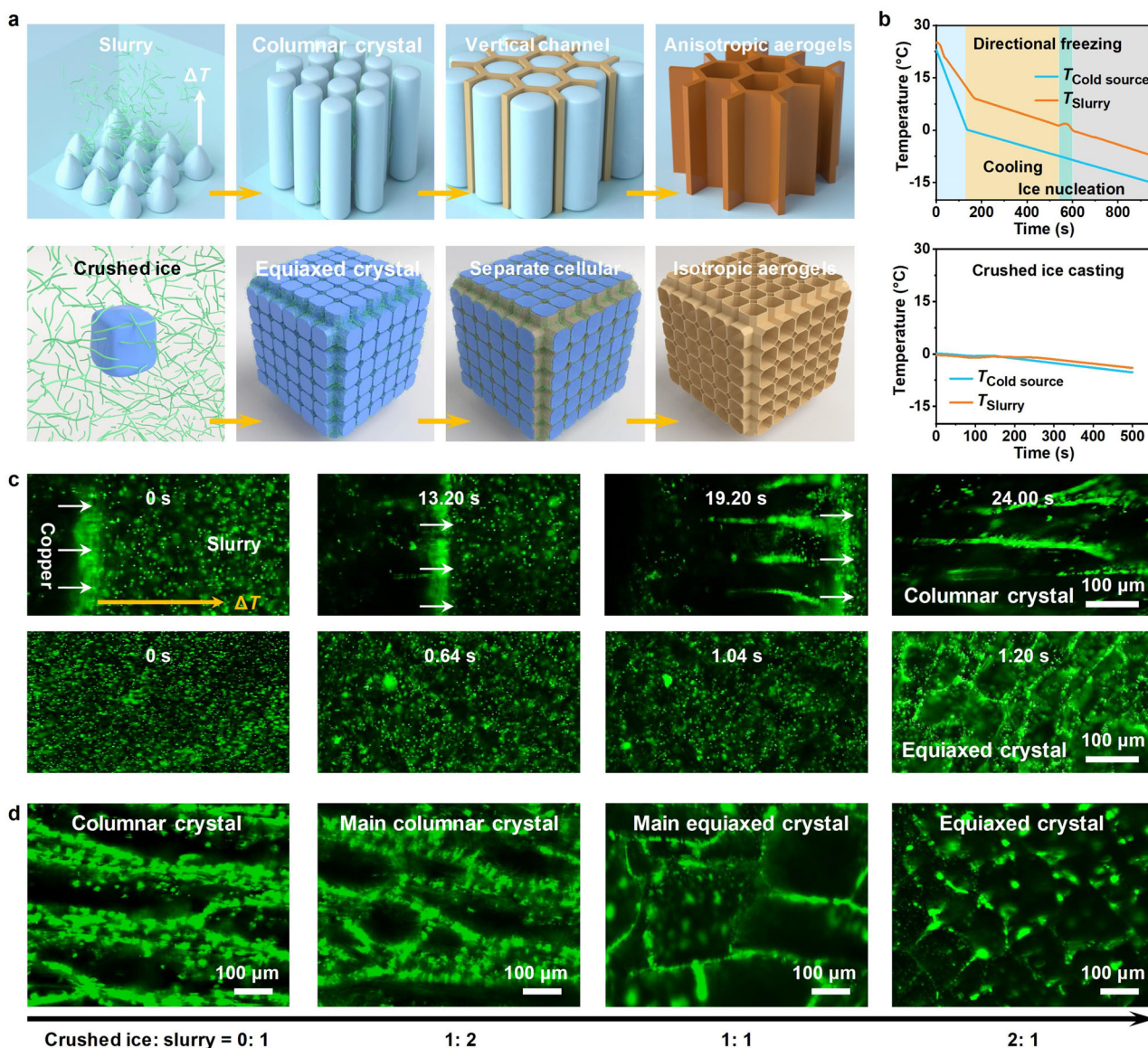
Fig. 2 | Proposed freezing mechanism. a Schematic illustration of the unidirectional freezing (upper) and CIC (bottom) processes. b Temperature variation over time during unidirectional freezing (upper) and CIC (bottom). c In situ observation
