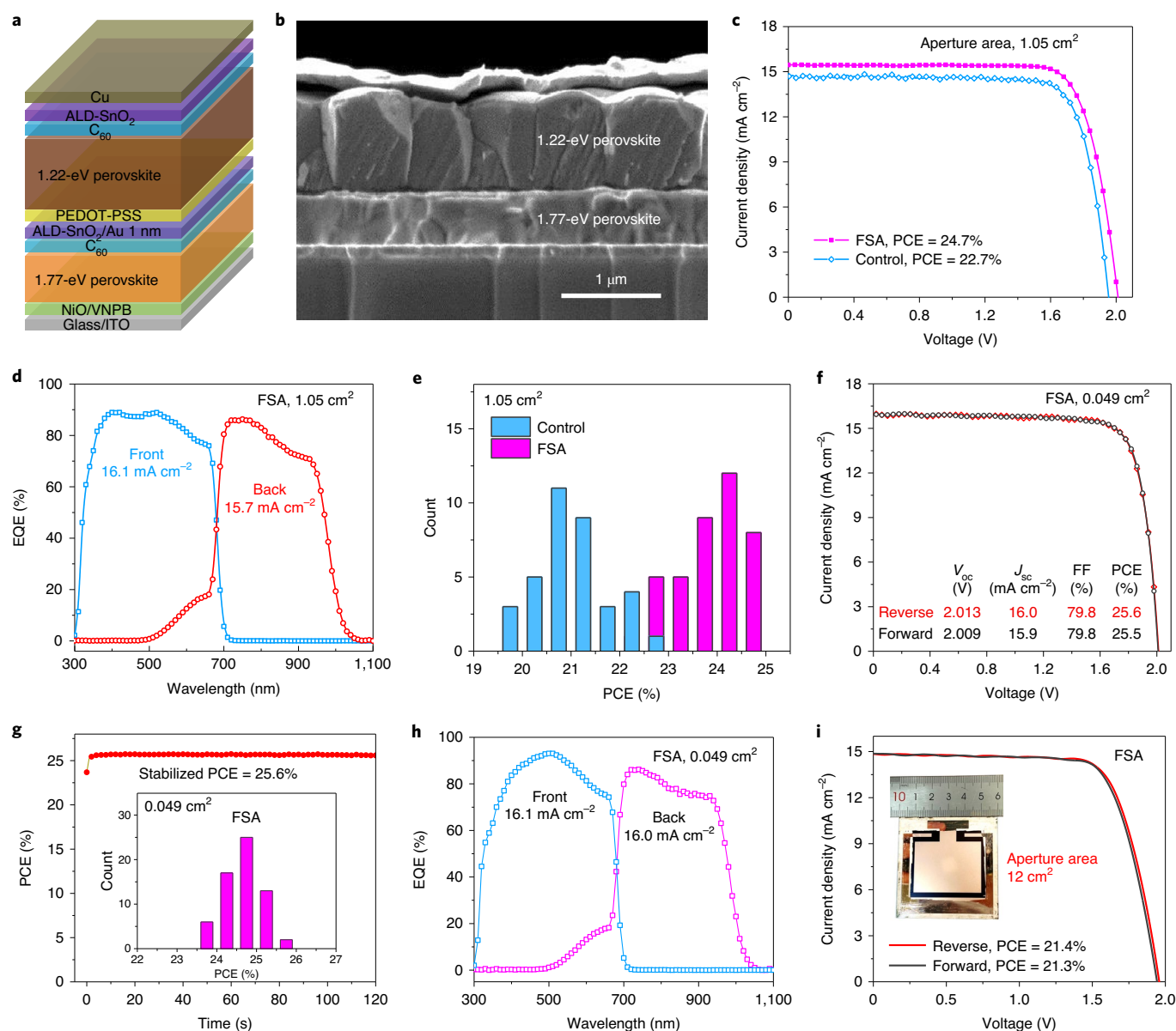
Fig. 4 | PV performance of monolithic all-perovskite tandem solar cells. a,b , Schematic structure ( a ) and cross-sectional scanning electron microscopy image ( b ) of all-perovskite tandem solar cell. c , J-V curves of the champion control and FSA tandem solar cells (aperture area, 1.05 cm 2 ). d , EQE curves of the champion FSA device. The front and back subcells show integrated J_{sc} values of 16.1 and 15.7 mA cm -2 , respectively. e , Histogram of PCEs for 36 control and 40 FSA tandem solar cells (1.05 cm 2 ). The devices show average PCEs of 21.1 ± 0.7% and 23.9 ± 0.6%, respectively. f , J-V curves of the champion FSA tandem cell with an aperture area of 0.049 cm 2 . g , Stabilized power output of the champion FSA tandem cell (0.049 cm 2 ). The inset shows the PCE distribution of 63 devices with an average PCE of 24.6 ± 0.4%. h , EQE curves of the champion FSA device (0.049 cm 2 ). The front and back subcells show integrated J_{sc} values of 16.1 and 16.0 mA cm -2 , respectively. i , J-V curves of an FSA tandem cell with an aperture area of 12 cm 2 . The inset shows the digital photo of the corresponding device. The device had a PCE of 21.4% under a reverse scan, with a V_{oc} of 1.958 V, J_{sc} of 14.8 mA cm -2 and FF of 73.8%.
