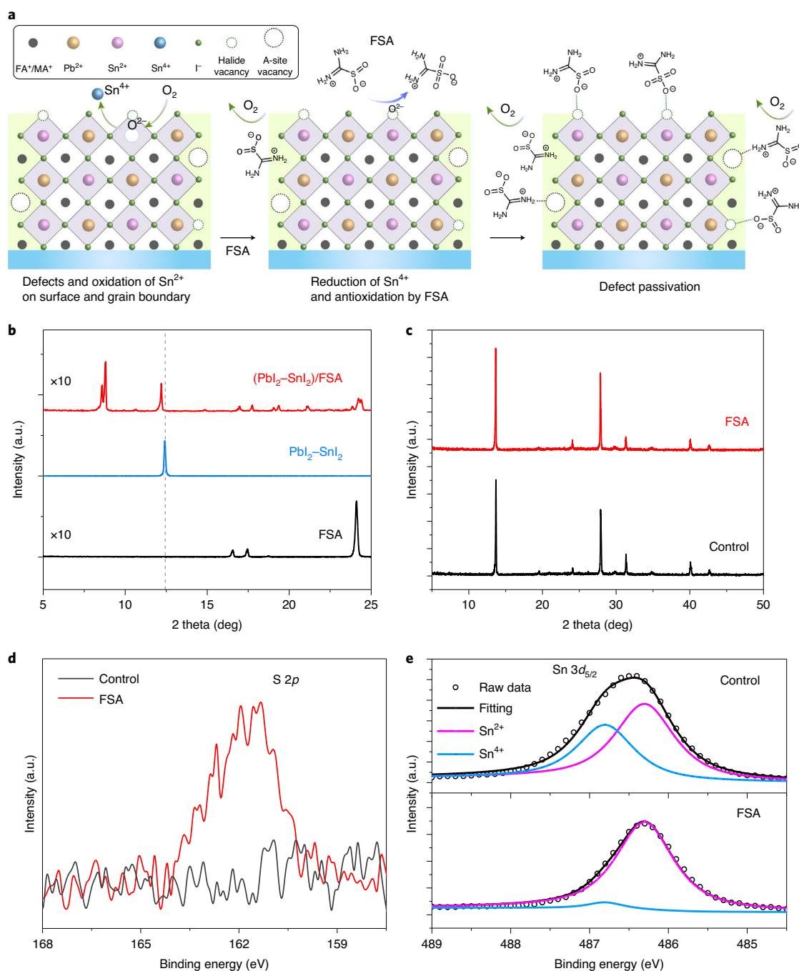
Fig. 1 | Characterization of mixed Pb-Sn narrow-bandgap perovskite films with FSA. a , Schematic illustration of antioxygenation and defect passivation at grain surfaces (including film surface and grain boundary) of mixed Pb-Sn perovskite films enabled by FSA. A-site represents the monovalent cation in the perovskites. b , X-ray diffraction patterns of FSA, a mixed Pb 1-x Sn x I 4 (1:1 in molar ratio) film and a (Pb 1-x Sn x ) 2 I 4 /FSA adduct film. The vertical dashed line indicates the diffraction peak position of the mixed Pb 1-x Sn x I 4 film. c , X-ray diffraction patterns of the control and FSA perovskite films. d , The S 2p XPS spectra of the control and FSA perovskite films. e , The Sn 3d 5/2 XPS spectra of the control and FSA perovskite films after exposure to air for ~10 min. The original spectra (points) and Gaussian-Lorentzian fitting curves (lines) are shown.
